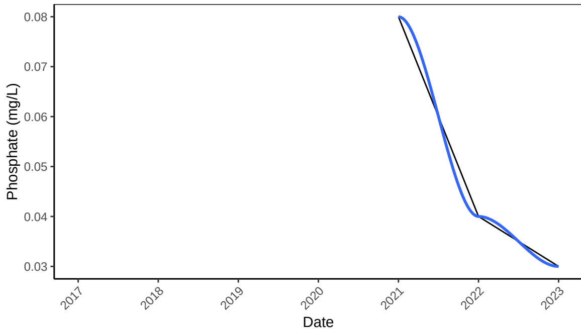
B2 Raceway 2 Phosphate (mg/L) Yearly Mean
